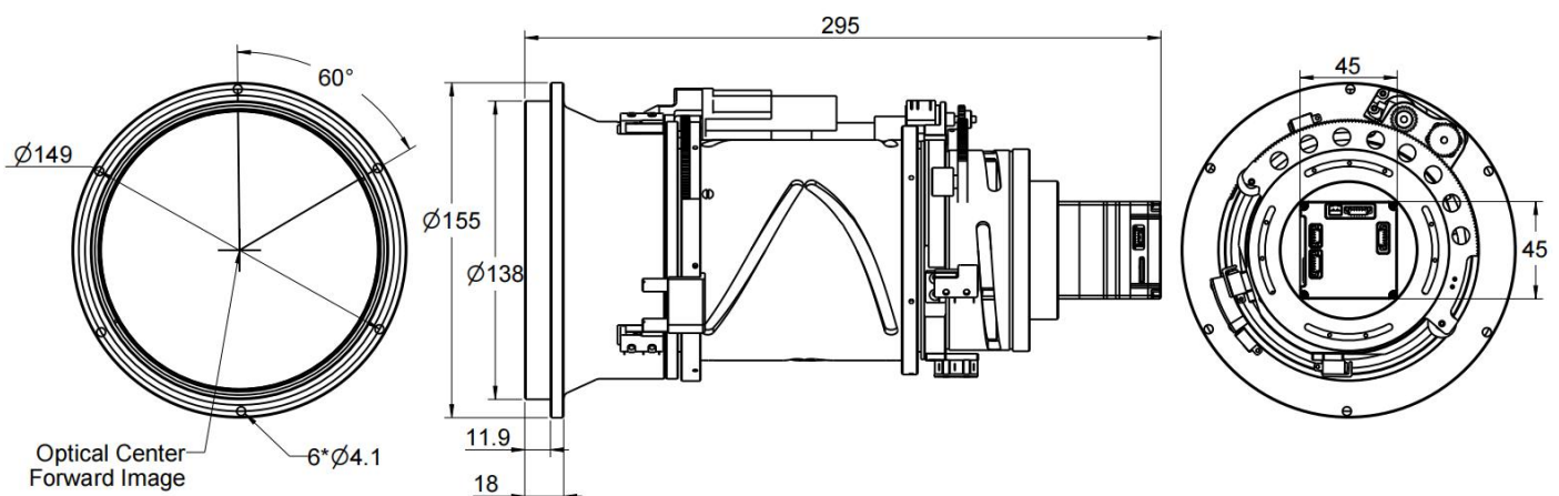
30~180mm Motorized Lens
