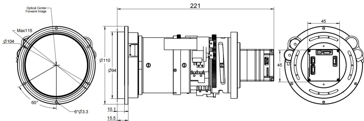
30~120mm Motorized Lens
